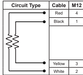
Dual 4-Wire Wiring
