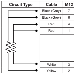
Dual 3-Wire Wiring
