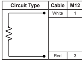
Single 2-Wire Wiring
