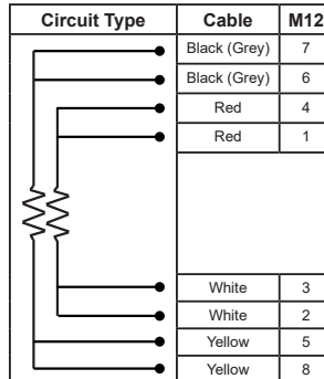
Dual 4-Wire Wiring
