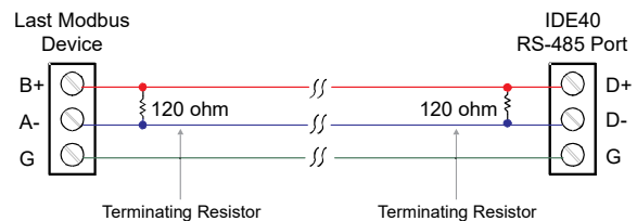
Figure 26. Serial Connections
