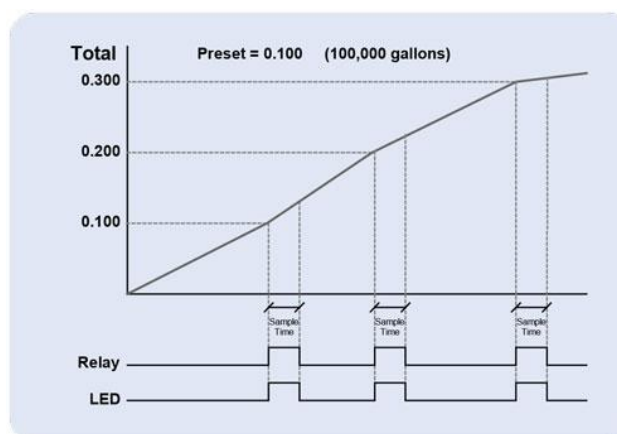
Figure 32. Total Relay Sampling Operation
