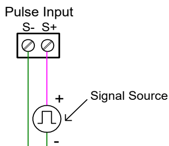
Figure 15. Flow Meter Pulse Input Connections
