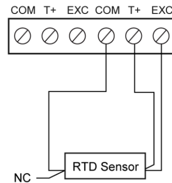
Figure 14. Four-Wire RTD Input Connections
