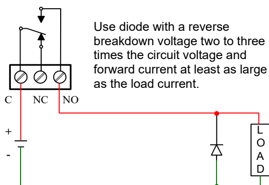
Figure 25. Low Voltage DC Loads Protection
