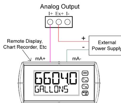
Figure 18. Passive 4-20 mA Output Powered by External Supply
