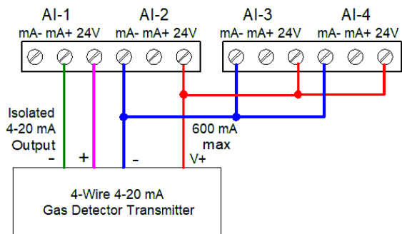
Figure 21. Powering 4-Wire Gas Detector & Isolated 4-20 mA Output
