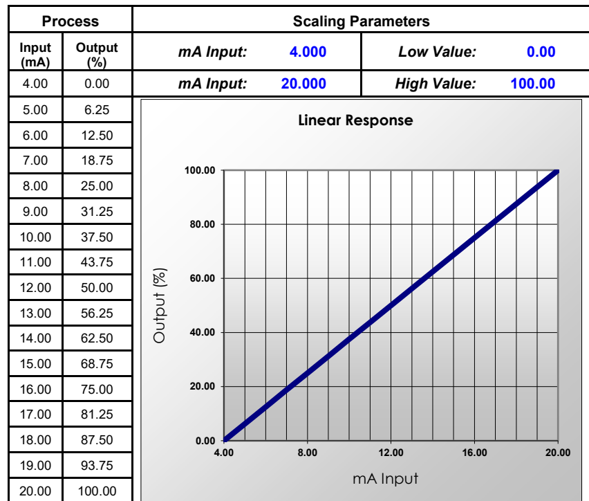
Figure 28. Linear Response Graph
