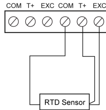
Figure 13. Three-Wire RTD Input Connections
