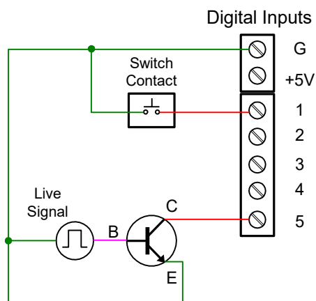
Figure 16. Digital Input from Switch Closure and Live Signal
