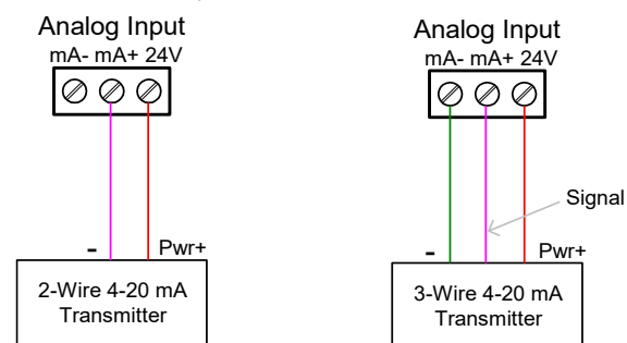
Figure 8. Transmitters Powered by IDE40 Isolated 24 VDC Power Supply
