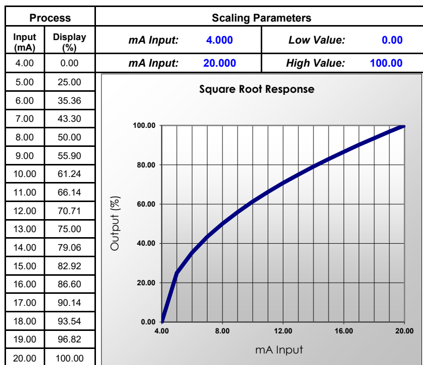
Figure 29. Square Root Response Graph
