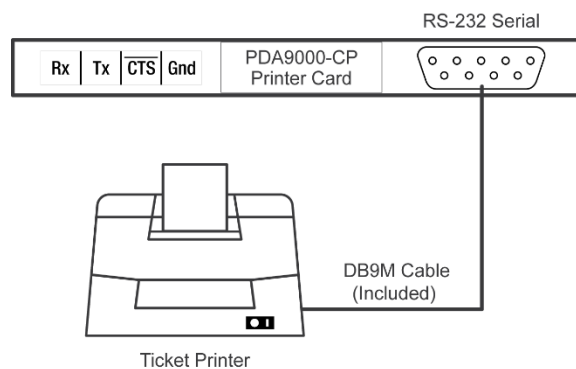
Figure 22. Printer Connections
