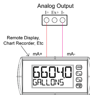
Figure 17. Active 4-20 mA Output Powered by Controller
