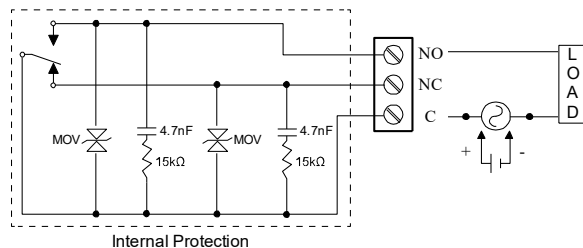
Figure 24. AC and DC Internal Inductive Loads Protection
