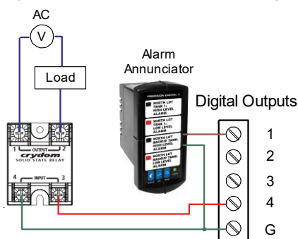
Figure 19. Digital Outputs Driving 5 V Solid State Relay
