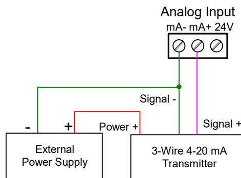
Figure 10. 3-Wire Transmitters Powered Externally
