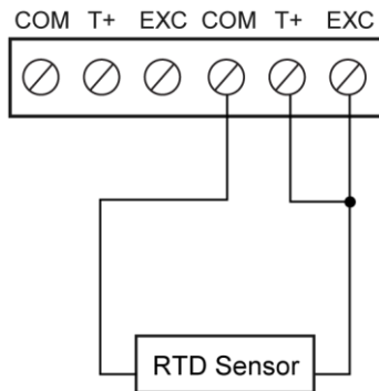
Figure 12. Two-Wire RTD Input Connections
