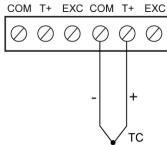
Figure 11. Thermocouple Input Connections
