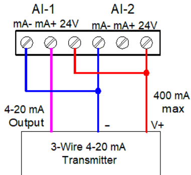
Figure 20. Two Supplies in Parallel Powering 3-Wire Transmitter
