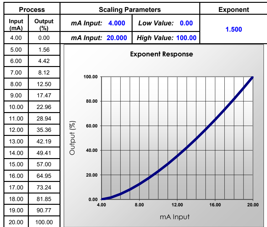
Figure 30. Exponent Response Graph
