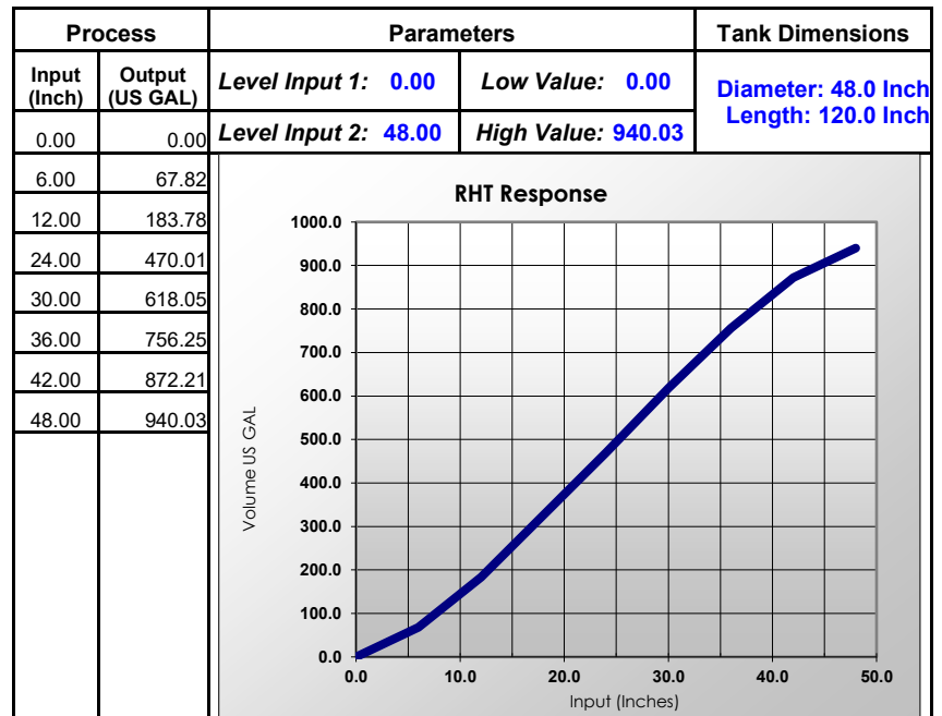
Figure 31. Round Horizontal Tank Volume Graph
