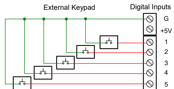
Figure 27. External Keypad Connections
