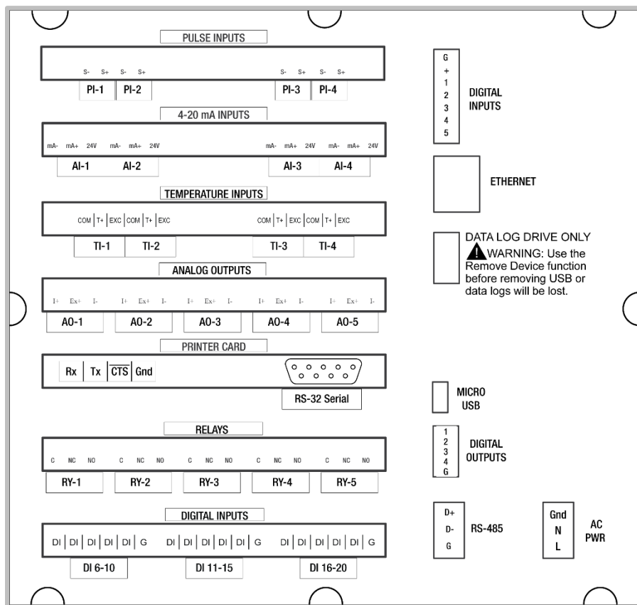
Figure 5. Connection Terminals for an IDE40-N-1-1A-1D-1P-1T-1O-1R-PR-ETH
