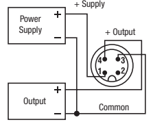
3 WIRE WIRING DIAGRAM EXAMPLE
