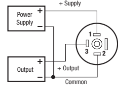
Wiring - M12 x 1 4-pin round connector
