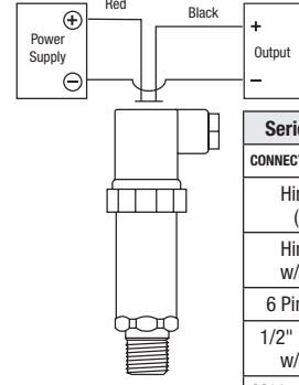
2 WIRE WIRING DIAGRAM EXAMPLE
