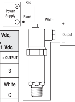
3 WIRE WIRING DIAGRAM EXAMPLE
