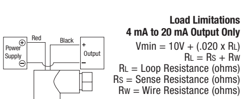
Wiring - M12 x 1 4-pin round connector
