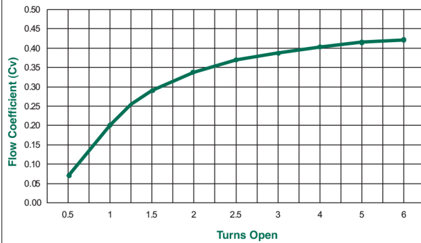
100 Series Mini Valve Flow Characteristics
