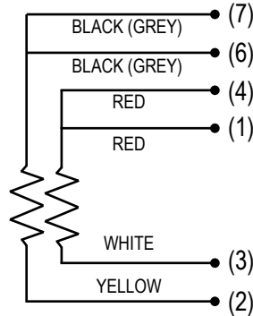
Dual 3-Wire
