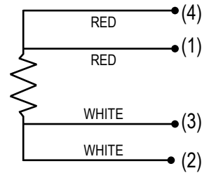
4-Wire
